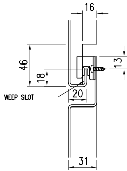
PANEL ABMESSUNGEN PANEL DIMENSIONS
