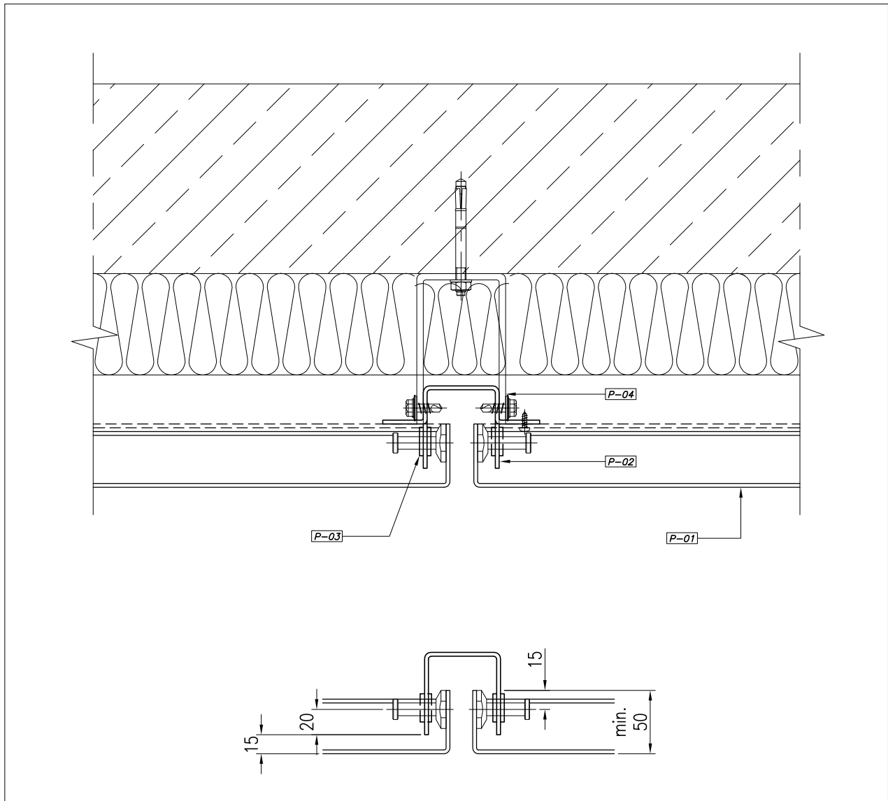
BOLZEN DETAIL PIN DETAIL
